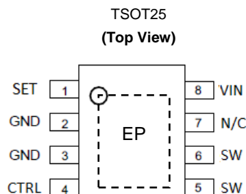
MSOP-8EP
