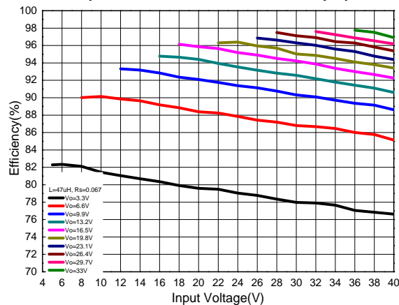
Efficiency vs. Input Voltage (MSOP-8EP, R_s=0.067\Omega , L=47\mu\text{H} )
