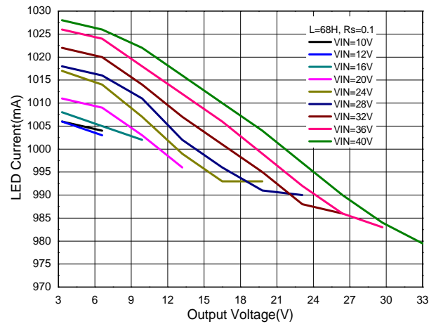
LED Current vs. Output Voltage (MSOP-8EP, R s =0.1Ω, L=68μH)
