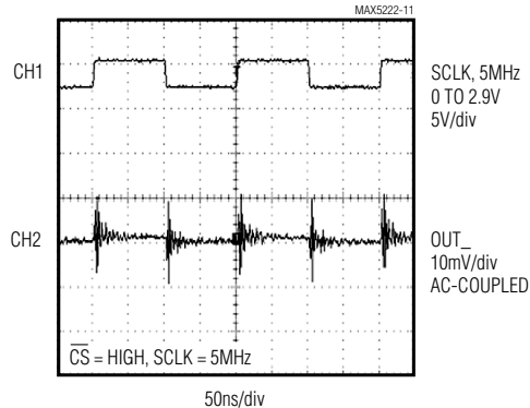
CLOCK FEEDTHROUGH
