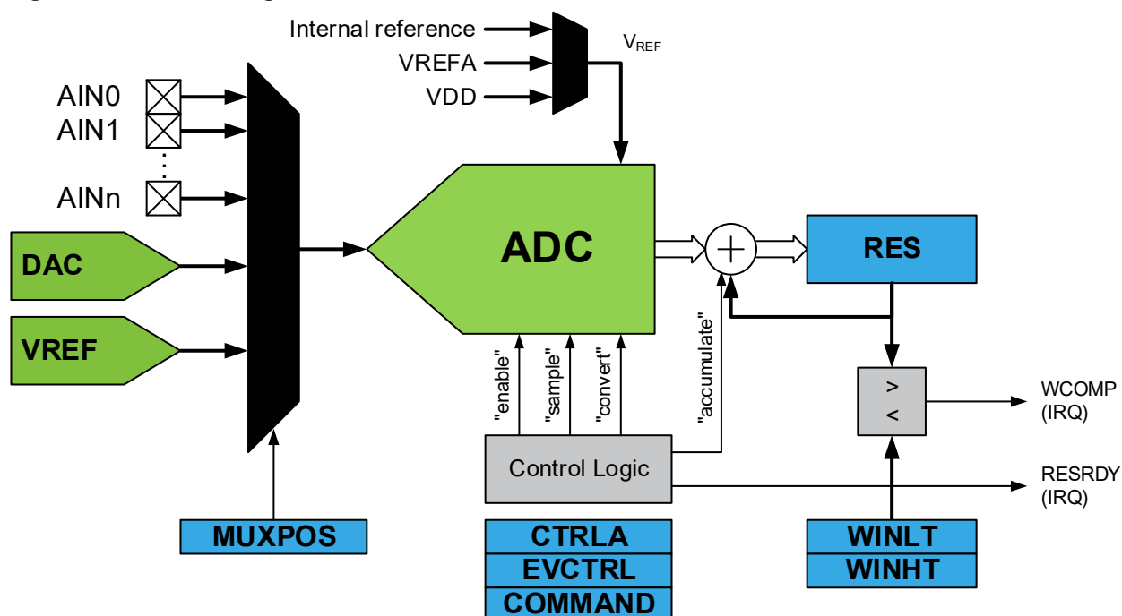
Figure 31-1. Block Diagram
