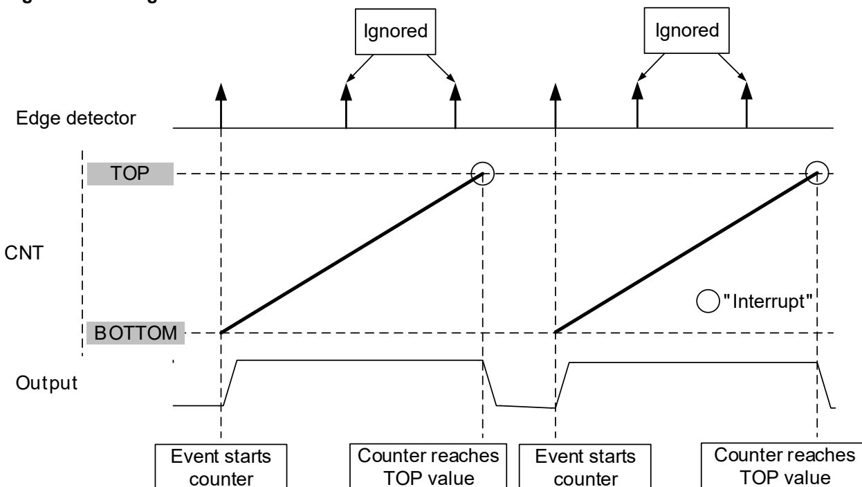
Figure 22-8. Single-Shot Mode
