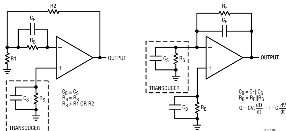
Figure 2. Noninverting and Inverting Gain Configurations
