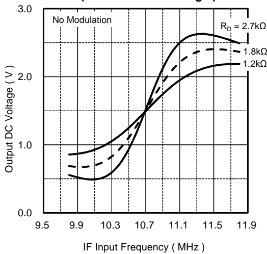
S-Curve Characteristics (DET OUT DC Voltage)
