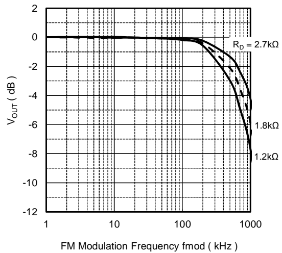
FM Demodulated Output Level vs. FM Modulation Frequency
