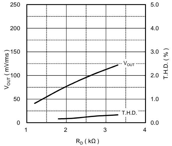
V_{\text{OUT}} , T.H.D. vs. R_D
