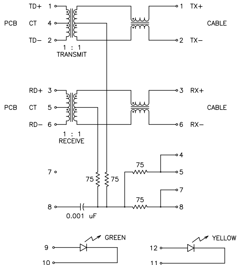
SCHEMATIC
