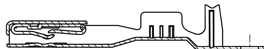
△ 2 SECT. B-B (SCALE 5:1)
