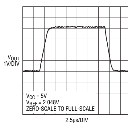
Large-Signal Response
