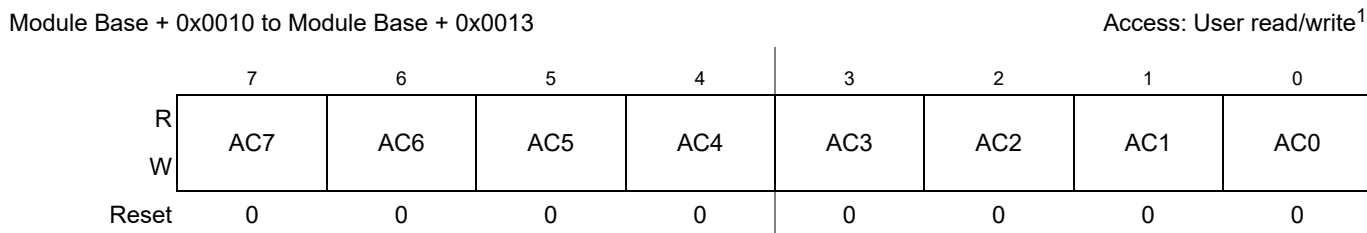
Figure 13-19. MSCAN Identifier Acceptance Registers (First Bank) — CANIDAR0–CANIDAR3
