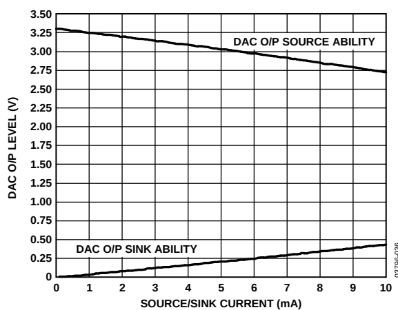
Figure 23. DAC Source and Sink Current Capability
