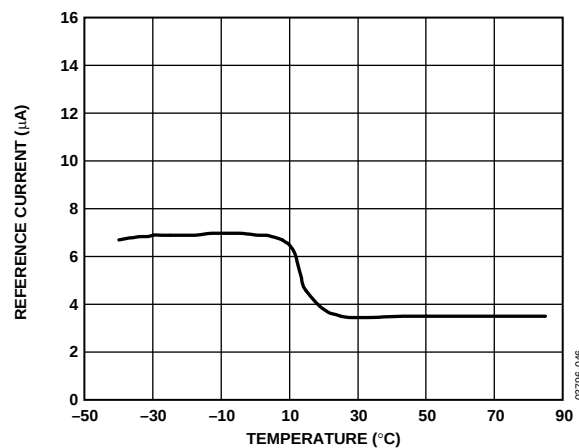
Figure 15. External Reference Current vs. Temperature
