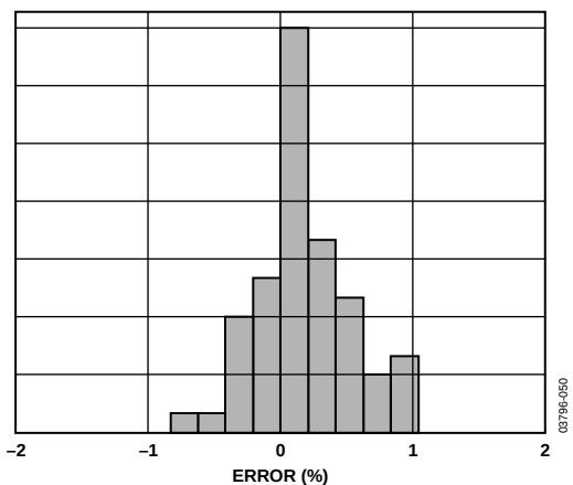
Figure 26. Typical Accuracy for Battery Channel ( 25^{\circ}\text{C} )
