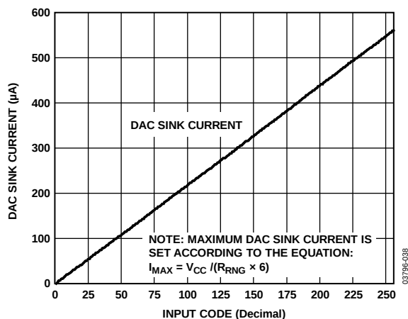
Figure 25. DAC Sink Current vs. Input Code with R_{\text{RNG}} = 1\text{ k}\Omega
