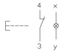
10 Illuminated pushbutton actuator single page 37
