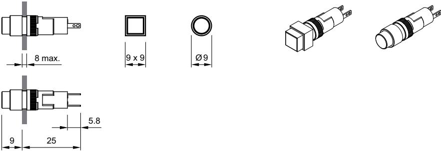
2 Illuminated pushbutton actuator page 109
