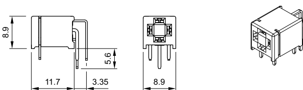
5 PCB plug-in base page 110
