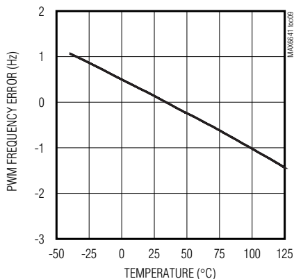
PWM FREQUENCY ERROR vs. DIE TEMPERATURE
