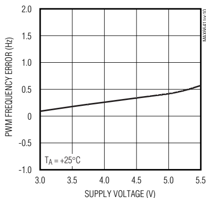
PWM FREQUENCY ERROR vs. SUPPLY VOLTAGE
