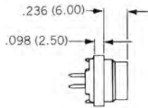
STRAIGHT VERSION
