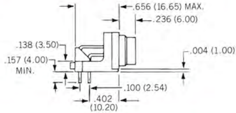
90° VERSION
