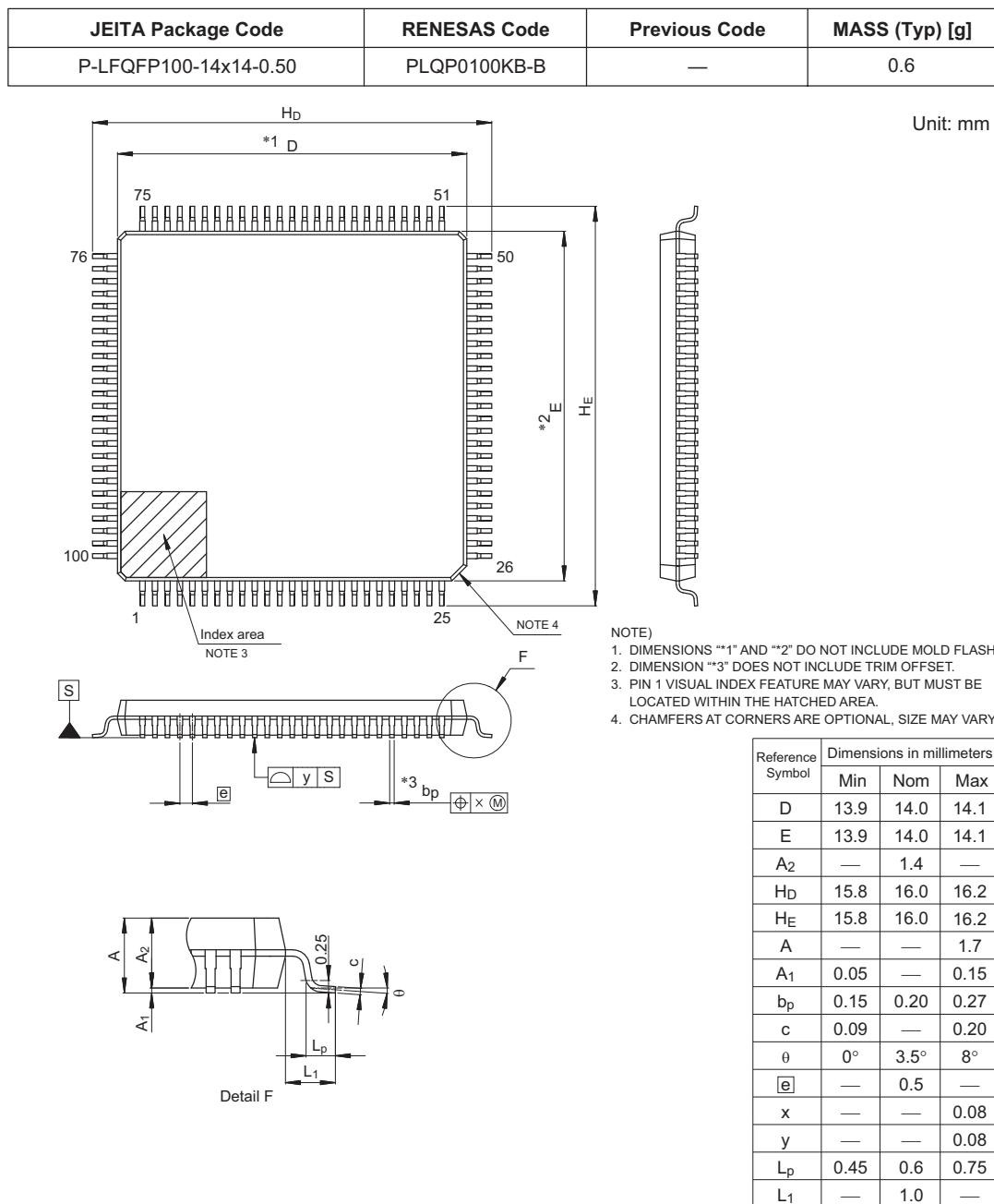
Figure 1.5 LQFP 100-pin
