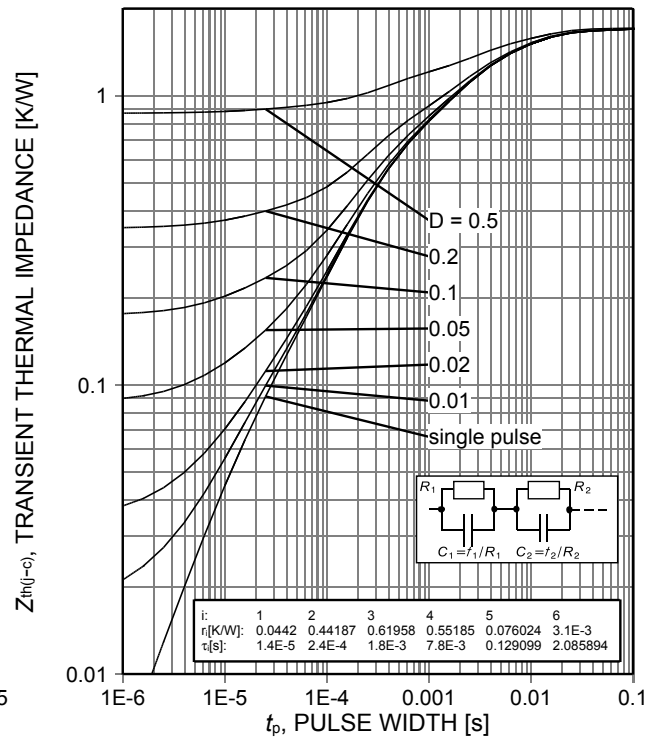
Figure 2. Diode transient thermal impedance per leg as a function of pulse width ( D = t_p/T )
