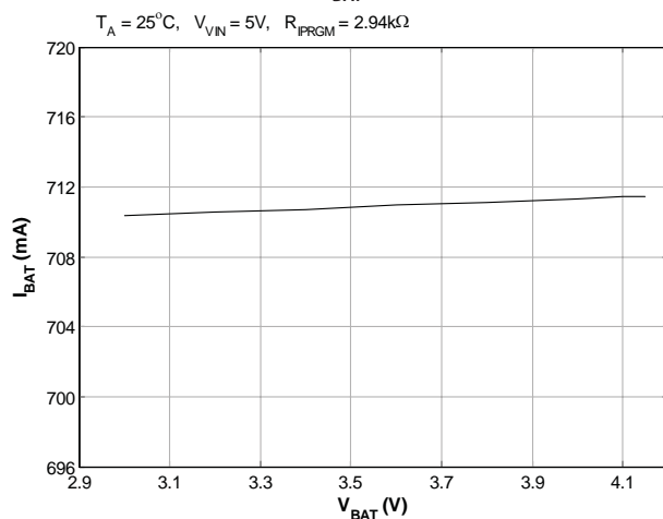
CC FQ V_{\text{BAT}} Regulation
