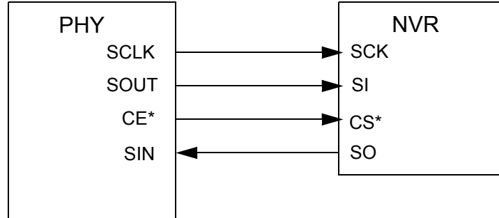
Figure 2-2 SPI Interface Block Diagram
