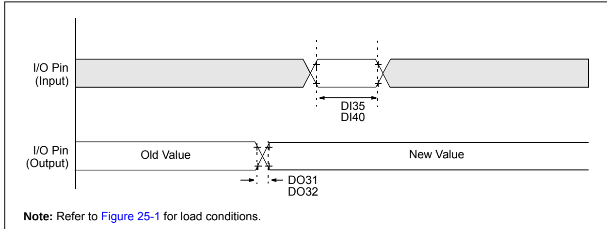
FIGURE 25-3: CLK0 AND I/O TIMING CHARACTERISTICS
