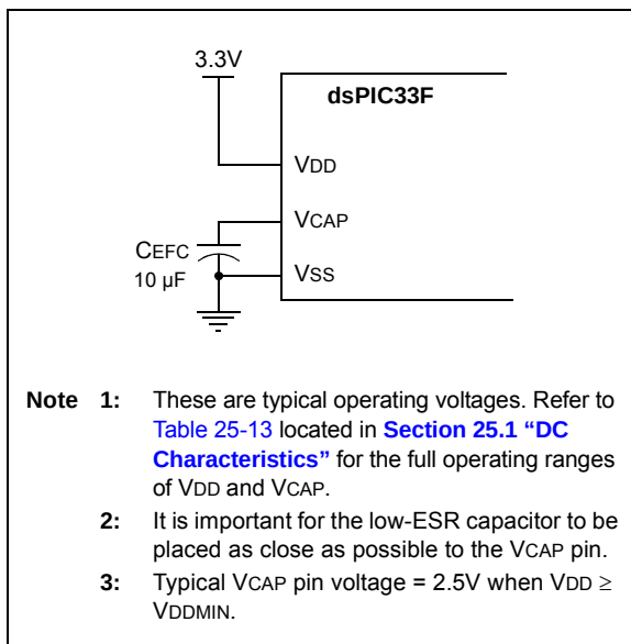
FIGURE 22-1: CONNECTIONS FOR THE ON-CHIP VOLTAGE REGULATOR (1,2,3)
