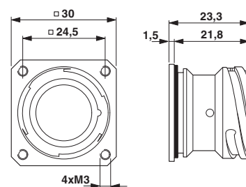
Dimensional drawing
