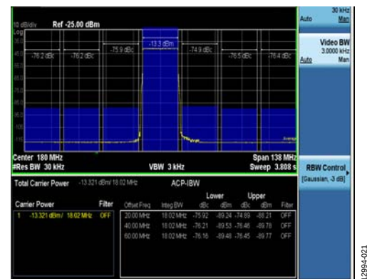
Figure 20. 1C 5 MHz Bandwidth LTE ACLR Performance, IF = 180 MHz, f_{DAC} = 1966.08 MHz
