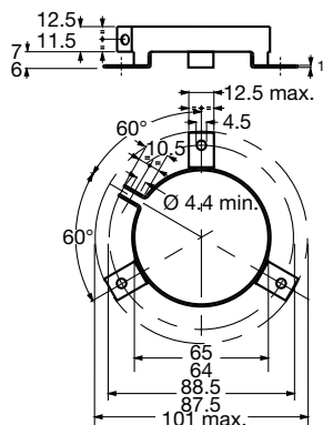
Fig. 3 - Dimensional outline of clamp for case Ø D = 65 mm
