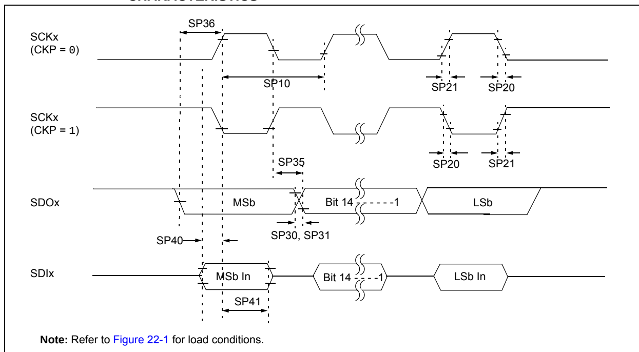
FIGURE 22-11: SPIx MASTER MODE (FULL-DUPLEX, CKP = 1, CKP = X, SMP = 1) TIMING CHARACTERISTICS
