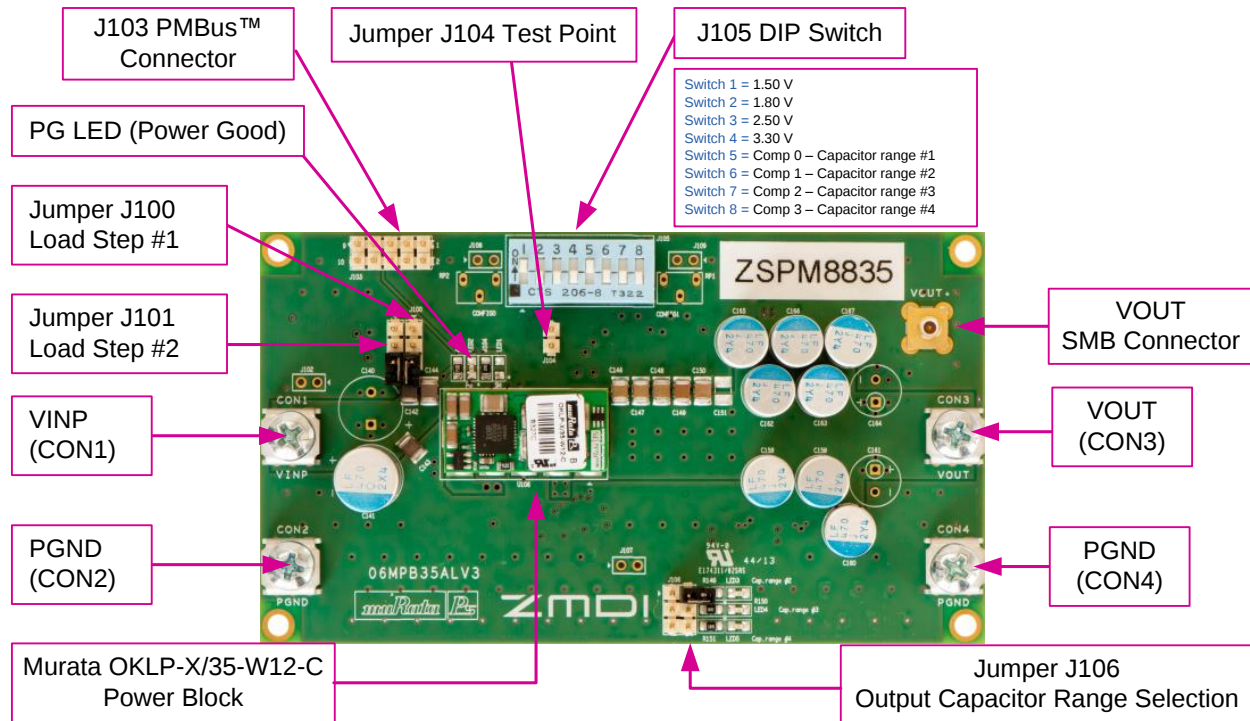
Figure 2.1 ZSPM8835-KIT Evaluation Board (Top Side)
