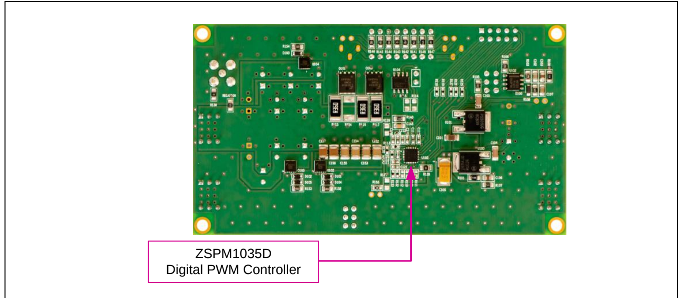
Figure 2.2 ZSPM8835-KIT Evaluation Board (Bottom Side)
