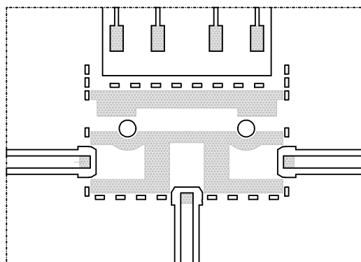
Area for solder paste
