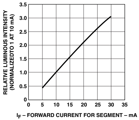
Figure 7. Relative luminous intensity vs. DC forward current.
