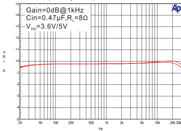
7. Frequency Response
