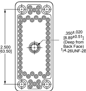
Receptacle Housing
