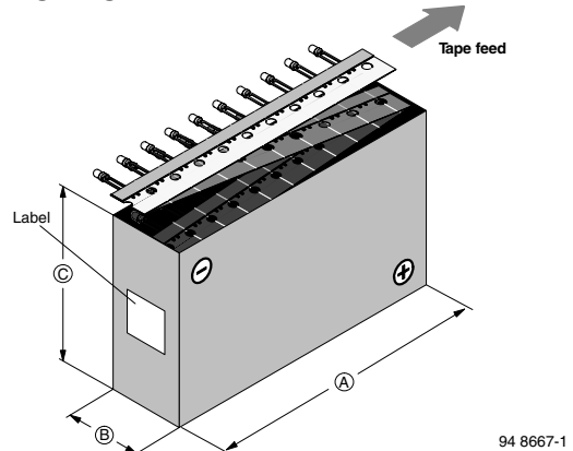
Figure 21. Tape Direction
