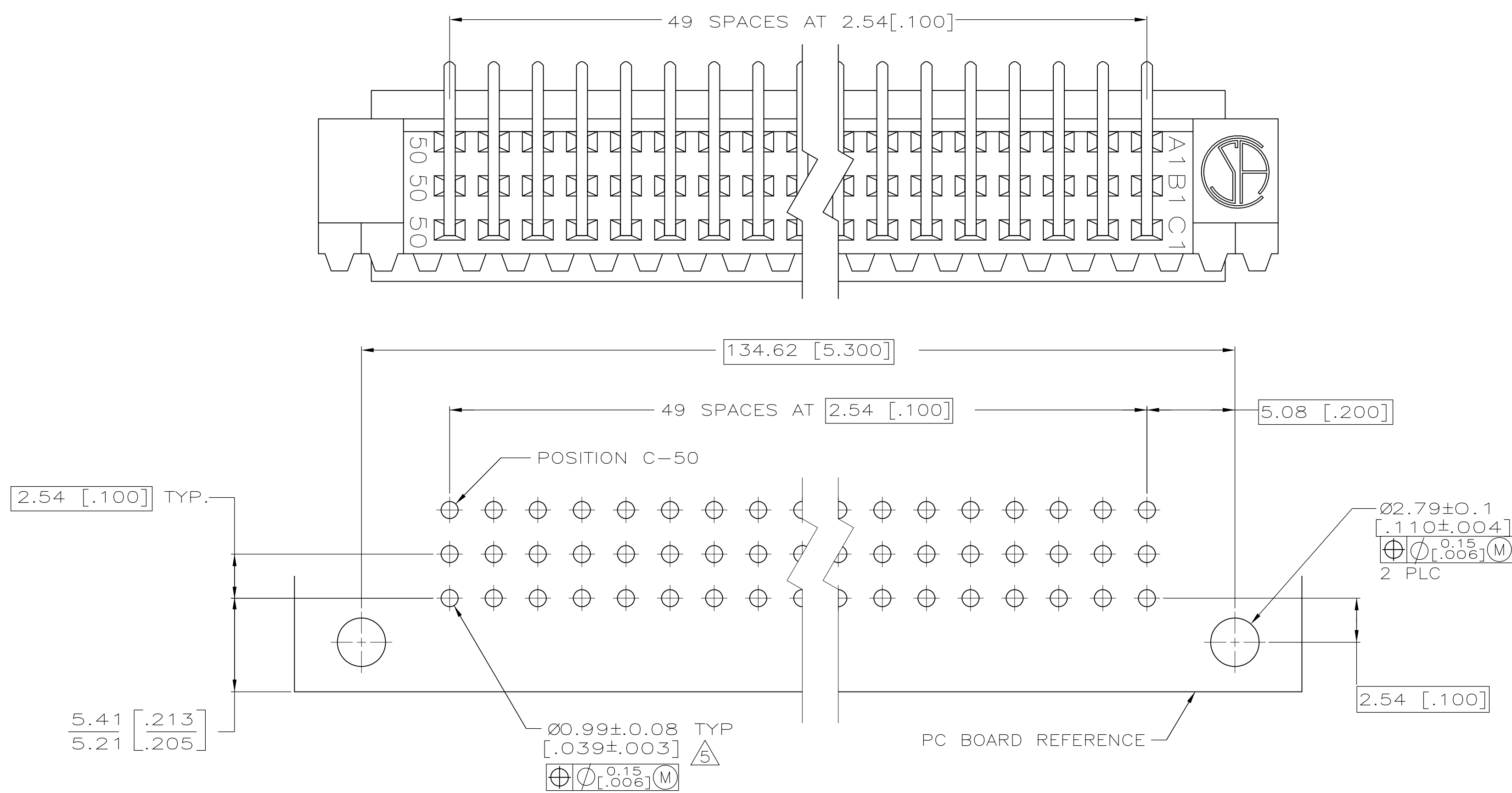
PC BOARD LAYOUT
