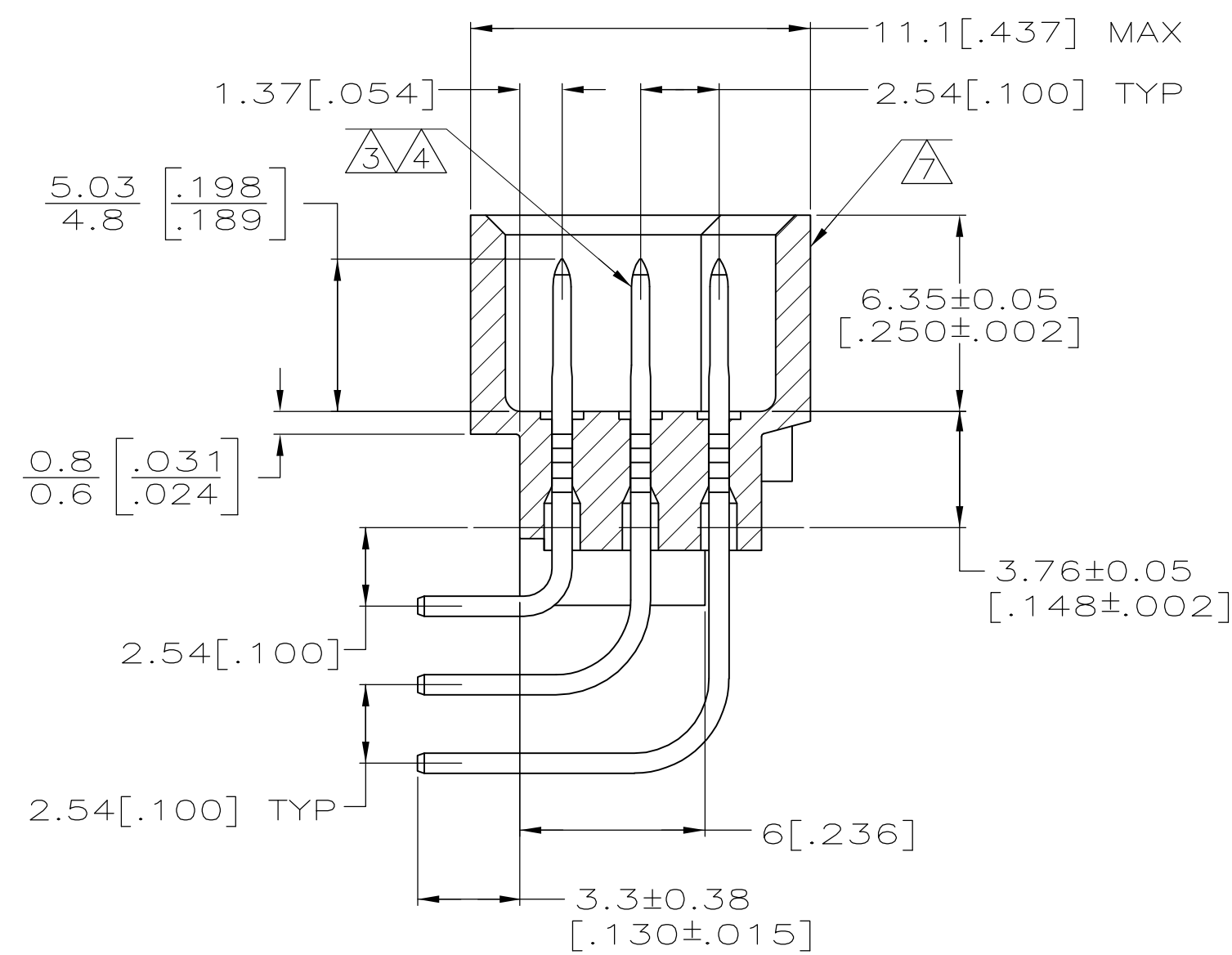
SECTION Z-Z
