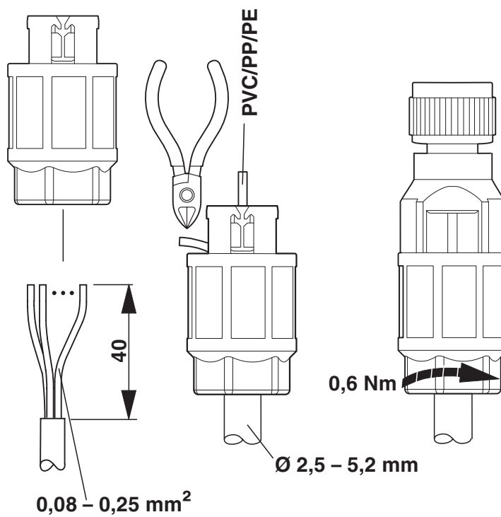
Functional drawing
