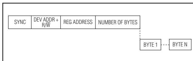
Figure 29. UART Read Packet
