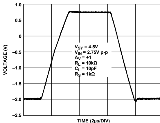
Figure 64. Large Signal Transient Response, V_{SY} = 4.5 V
