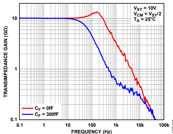
Figure 129. Transimpedance Gain vs. Frequency
