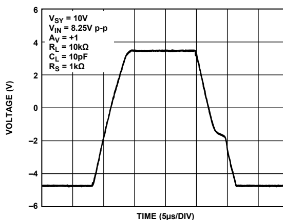
Figure 65. Large Signal Transient Response, V_{SY} = 10 V
