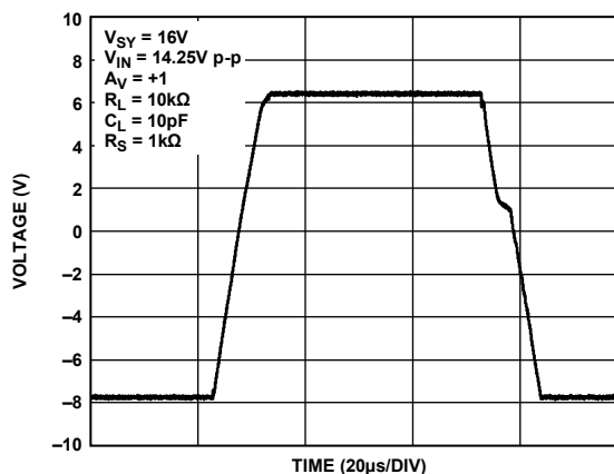
Figure 66. Large Signal Transient Response, V_{SY} = 16 V
