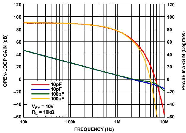
Figure 55. Open-Loop Gain and Phase Margin vs. Frequency
