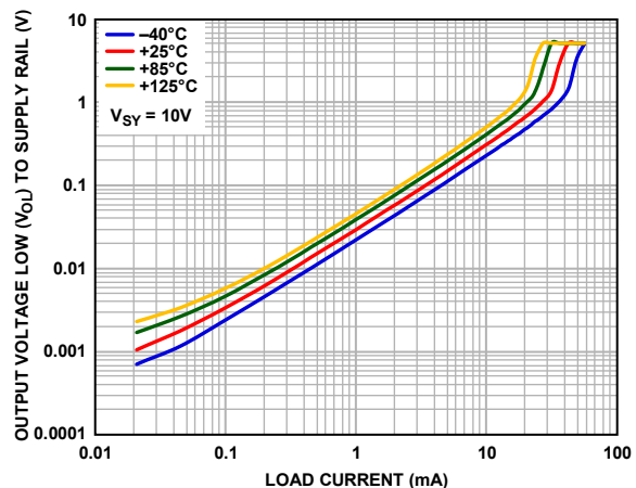
Figure 41. Output Voltage Low ( V_{OL} ) to Supply Rail vs. Load Current ( I_{LOAD} ), V_{SY} = 10\text{ V}
