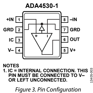
Figure 3. Pin Configuration
