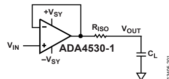
Figure 101. Stability Compensation with Isolating Resistor, R_{ISO}
