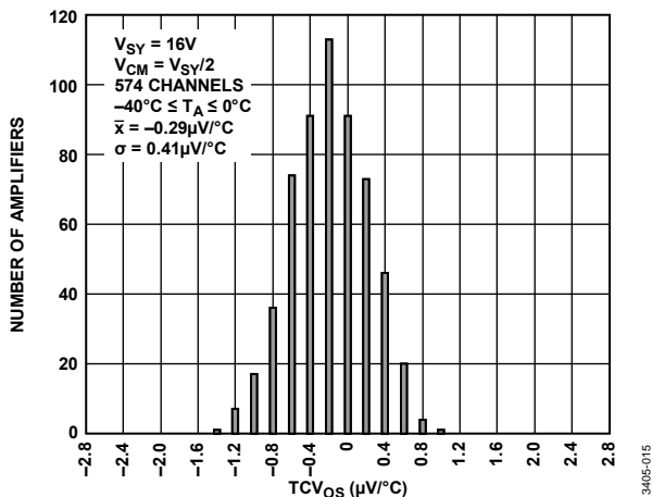
Figure 12. Input Offset Voltage Drift Distribution, -40^{\circ}\text{C} \leq T_A \leq 0^{\circ}\text{C} , V_{SY} = 16\text{ V}
