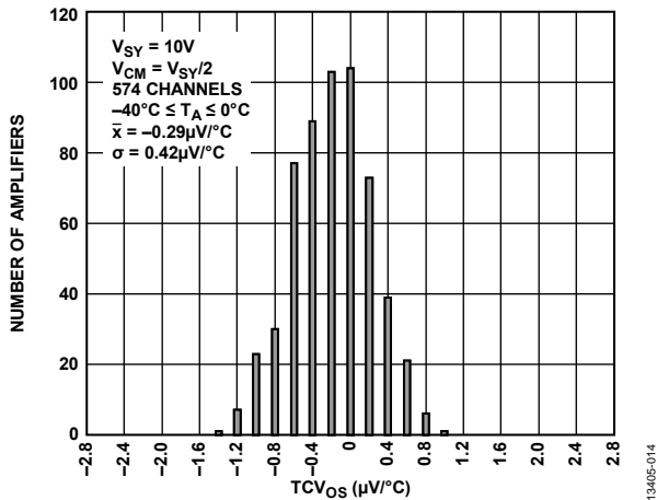
Figure 11. Input Offset Voltage Drift Distribution, -40^{\circ}\text{C} \leq T_A \leq 0^{\circ}\text{C} , V_{SY} = 10\text{ V}
