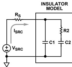
Figure 108. Dielectric Relaxation Model Test Circuit
