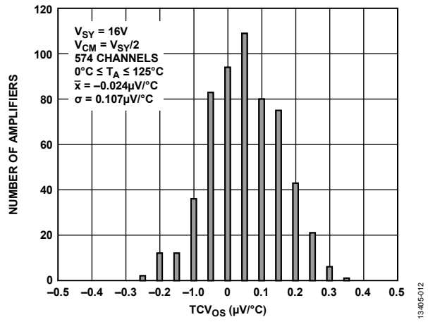
Figure 15. Input Offset Voltage Drift Distribution, 0^{\circ}\text{C} \leq T_A \leq 125^{\circ}\text{C} , V_{SY} = 16\text{ V}
