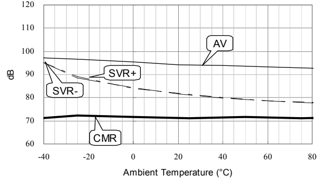
Amp.Gain vs. Ambient Temperature ( Ach )
