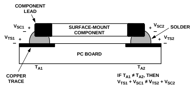
Figure 70. Mismatch in Seebeck Voltages Causes Seebeck Voltage Error
