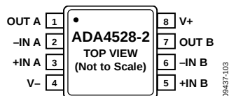
Figure 6. ADA4528-2 Pin Configuration, 8-Lead MSOP
