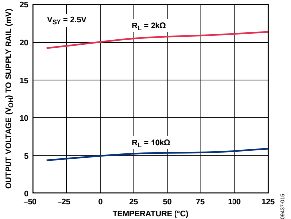
Figure 21. Output Voltage ( V_{OH} ) to Supply Rail vs. Temperature
