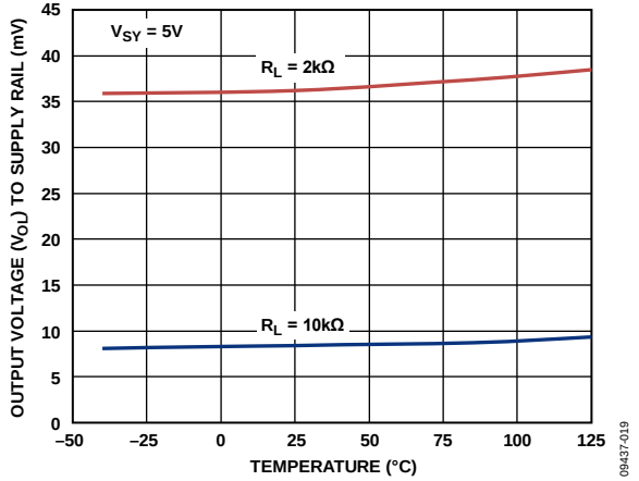
Figure 23. Output Voltage ( V_{OV} ) to Supply Rail vs. Temperature
