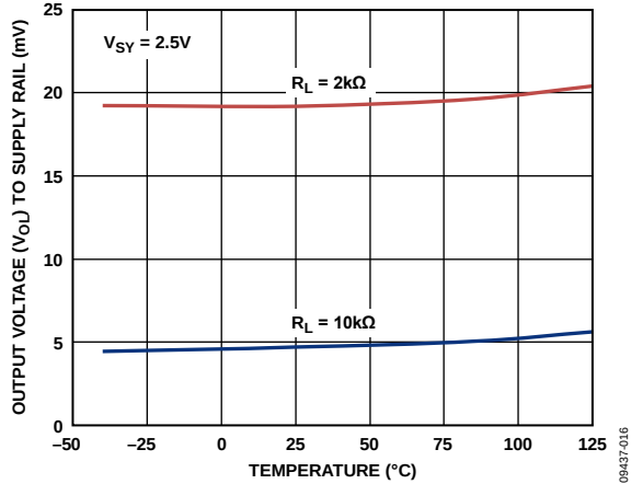
Figure 20. Output Voltage ( V_{OV} ) to Supply Rail vs. Temperature
