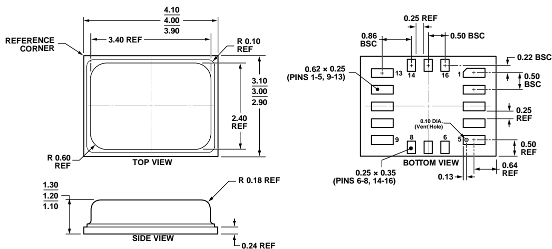
Figure 67. 16-Terminal Chip Array, Small Outline, No Lead Cavity [LGA_CAV] 4.00 mm x 3.00 mm x 1.2 mm Body (CE-16-3) Dimensions shown in millimeters
