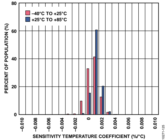
Figure 26. Y-Axis Sensitivity Temperature Coefficient, V_s = 2.5 V
