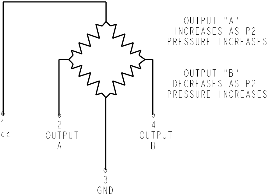
CIRCUIT DIAGRAM
