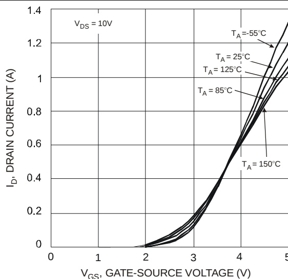
Fig. 11 Transfer Characteristics
