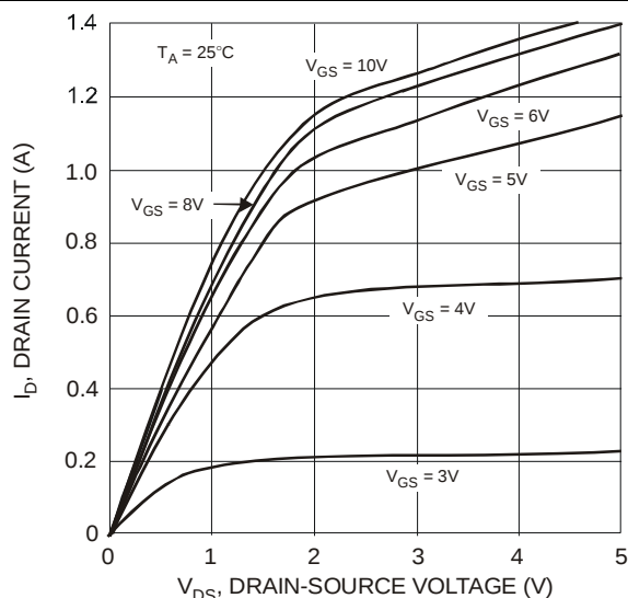
Fig. 10 Output Characteristics
