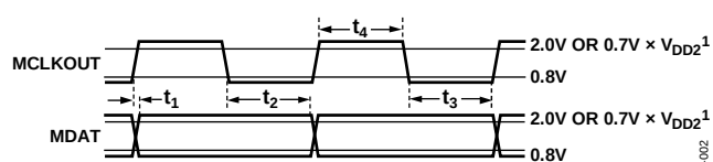
Figure 2. Data Timing
