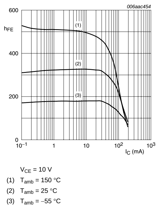
Fig 6. 2PD601BSL: DC current gain as a function of collector current; typical values
