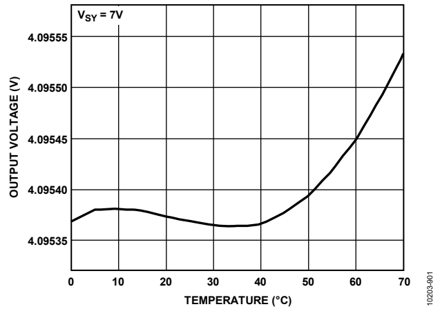
Figure 69. ADR4540 C Grade Output Voltage vs. Temperature
