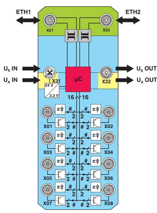
Figure 1 Internal wiring of connections
