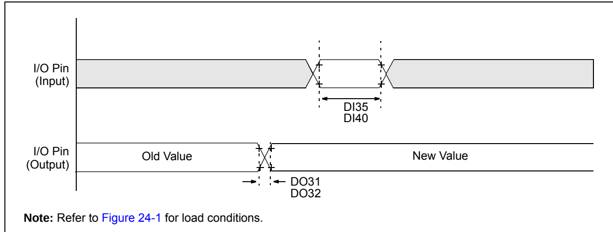
FIGURE 24-3: CLK0 AND I/O TIMING CHARACTERISTICS
